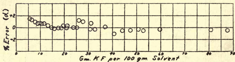
Figure 5. Determination of Ethyl Alcohol in the Presence of Methyl Alcohol.
